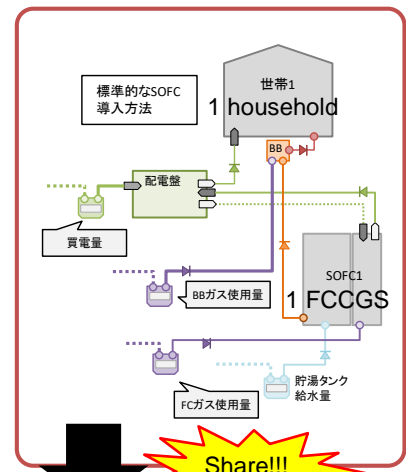
Fig1 Fuel Cell for Residence
